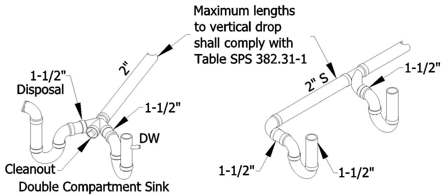
Drawing 31d
