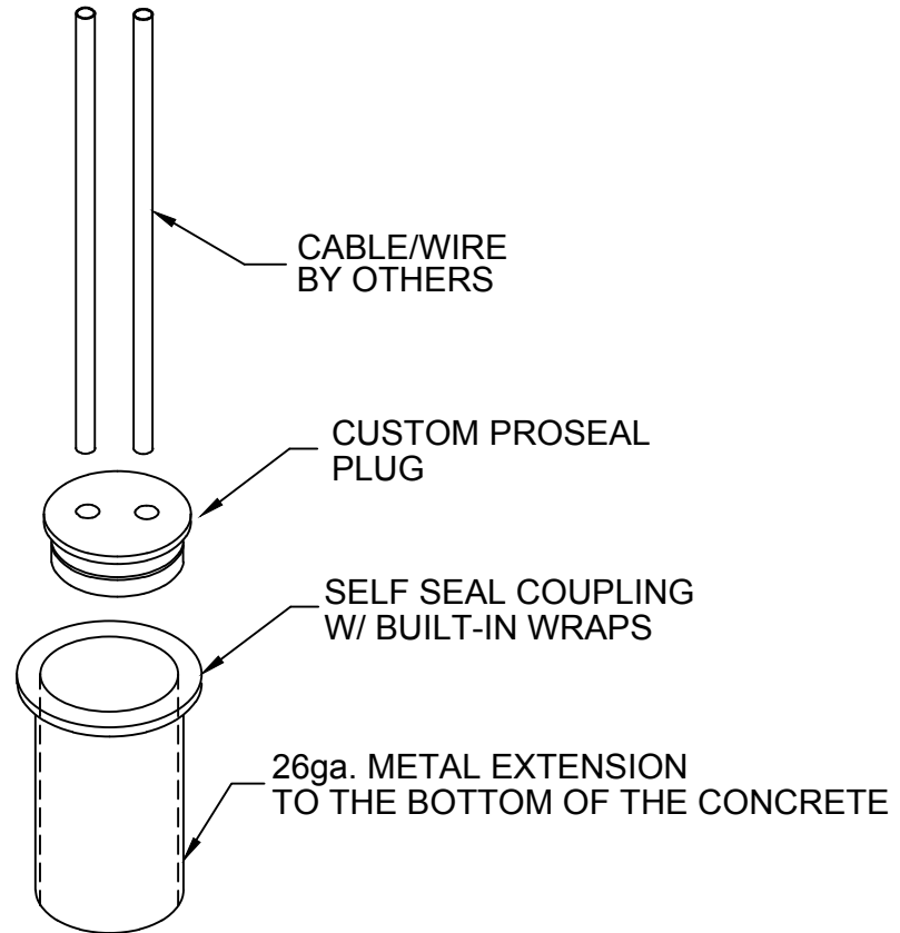
EXPLODED VIEW
