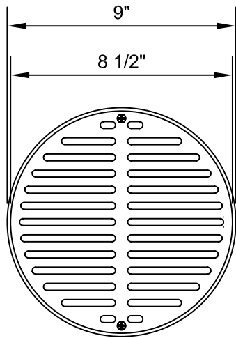
X.H. CAST IRON GRATE
