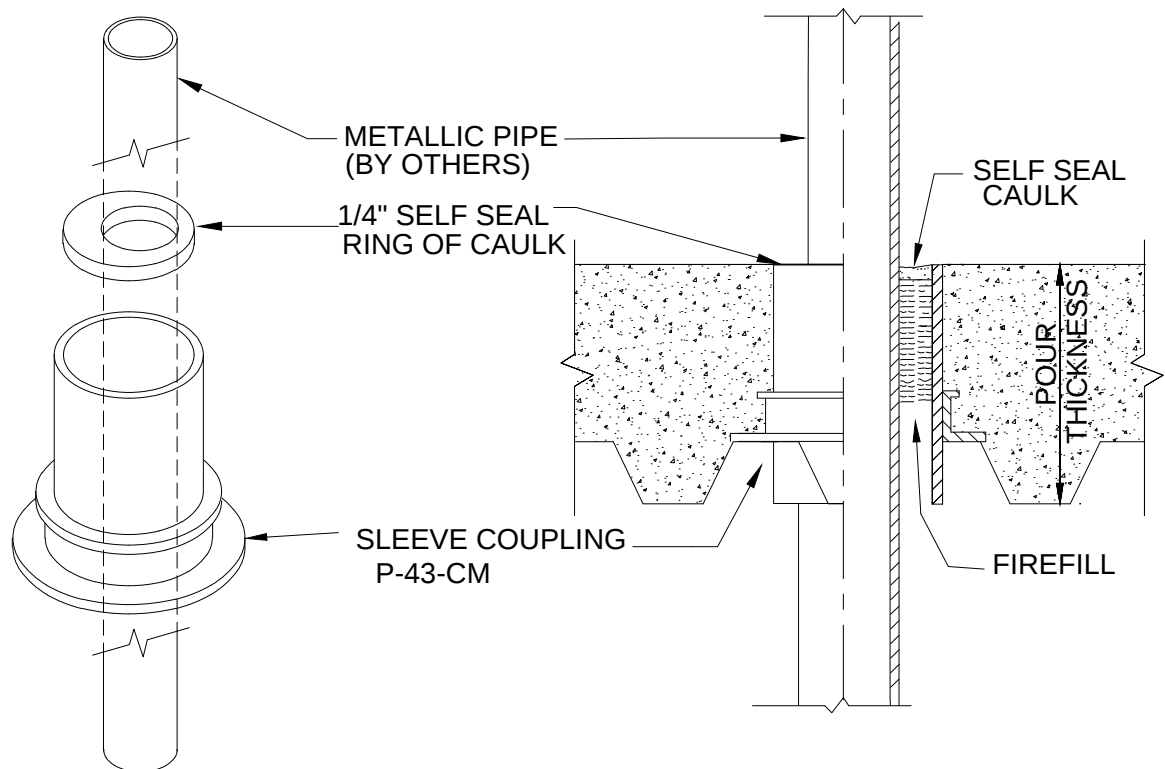
EXPLODED VIEW
