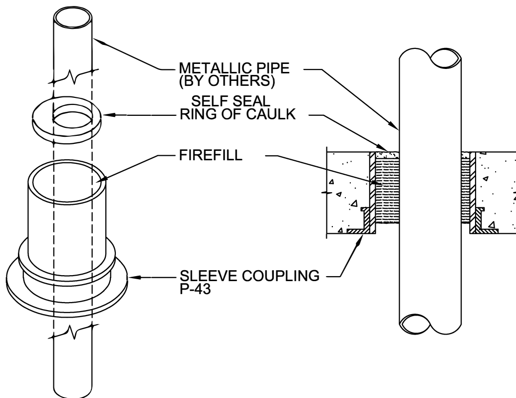
EXPLODED VIEW
