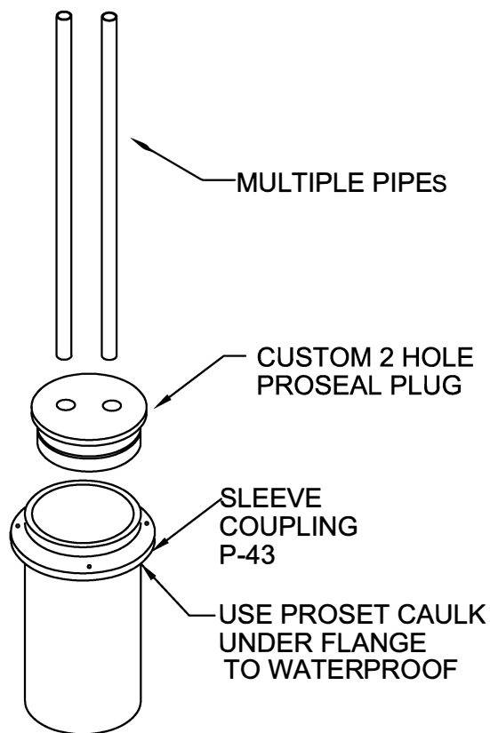
EXPLODED VIEW
