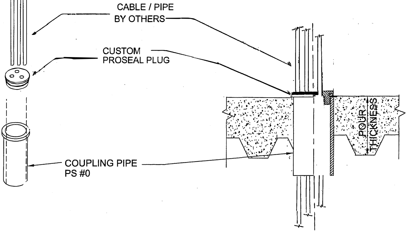
EXPLODED VIEW
