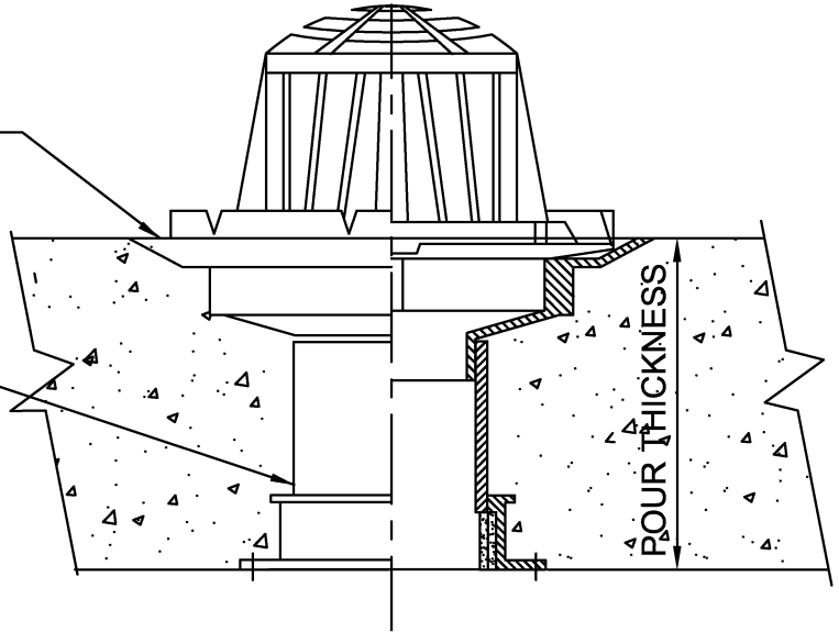
DOMED ROOF DRAIN P-67 PS #20
