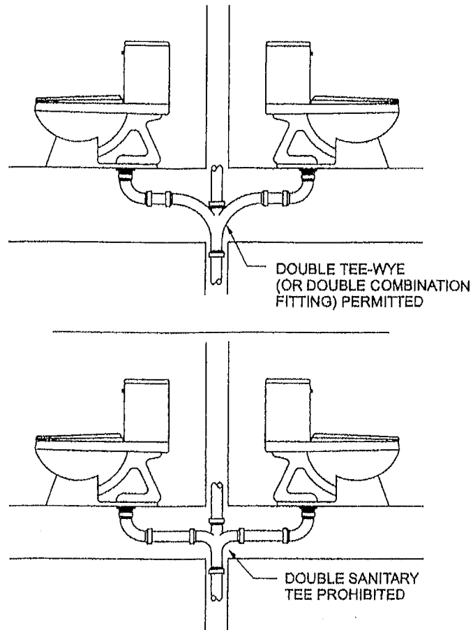
FIGURE 7.1 Back-to-back blowout fixtures. Copyright 2002, International Code Council, Inc., Falls Church, Virginia. Reproduced with permission. All rights reserved.
